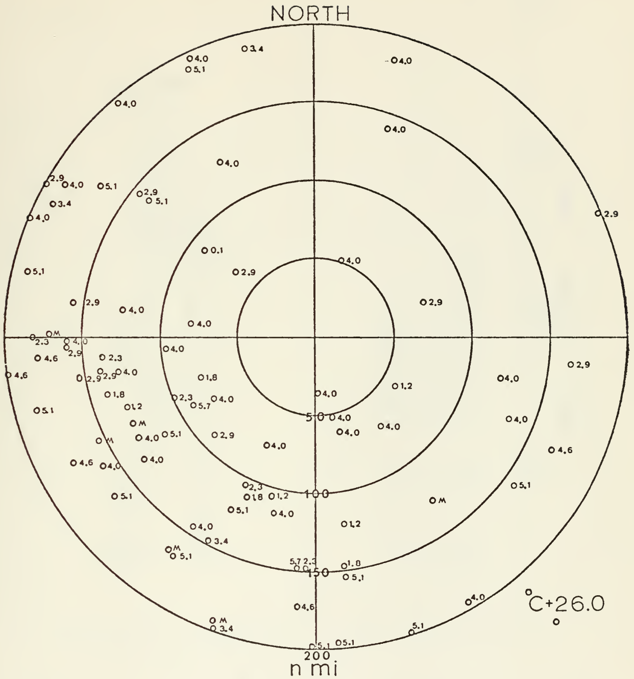
Figure 8. Composite of Observed Sea-Surface Temperatures for Hurricane Camille--150000GMT AUG - 171800GMT AUG 1969.
